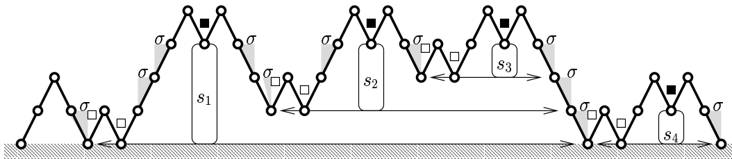
FIGURE 6. A representative of a set of bicolored black-isolated paths
