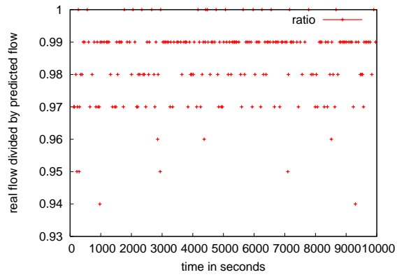
Figure 8. Accuracy of the HTM during scenario (a) scheduled with MSF, on spinnaker on the top and artimon on the bottom
