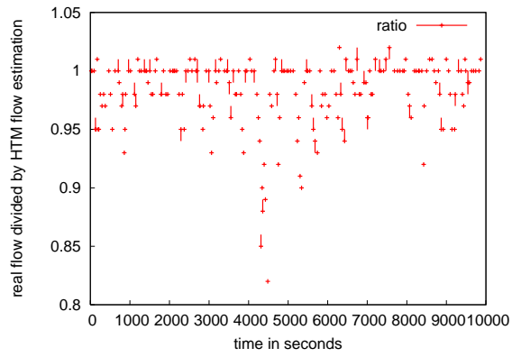
Figure 3. Accuracy of the HTM during scenario (a), \mu = 20 seconds, scheduled with HMCT, on spinner on the top and artimon on the bottom
