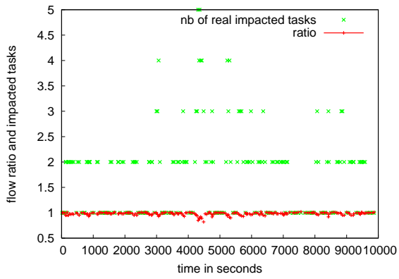
Figure 3. Accuracy of the HTM during scenario (a), \mu = 20 seconds, scheduled with HMCT, on spinner on the top and artimon on the bottom
