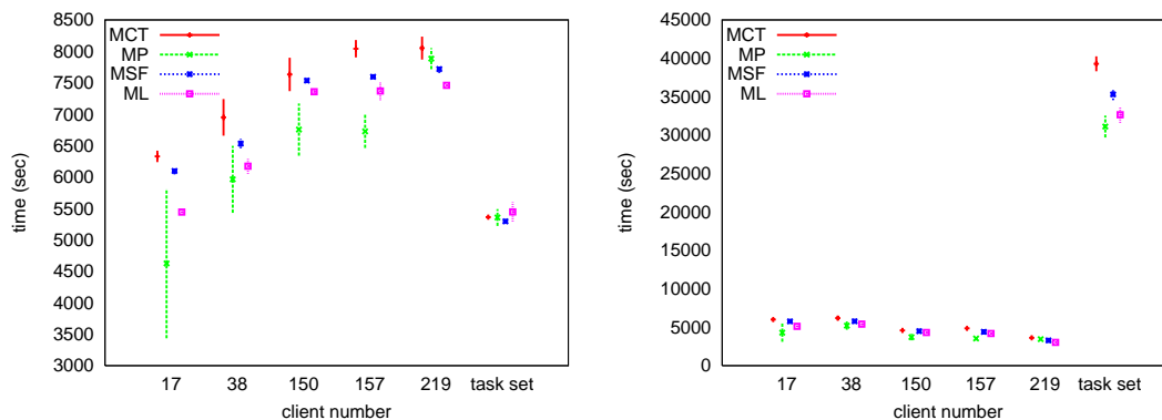
Figure 18. Scenario (d'): results on the makespan and on the sumflow for the third experiment
