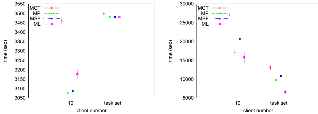
Figure 22. Scenario (h'): makespan and sumflow results for the third experiment
