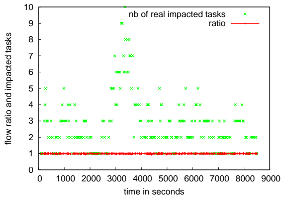
Figure 4. Accuracy of the HTM during scenario (a'), \mu = 17 seconds, scheduled with HMCT, on spinner on the top and artimon on the bottom
