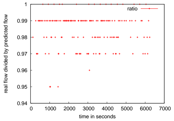
Figure 15. Accuracy of the HTM during scenario (j'), \mu = 20 seconds, scheduled with MSF, on spinner on the top and artimon on the bottom
