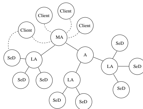
Figure 2: DIET Architecture.
