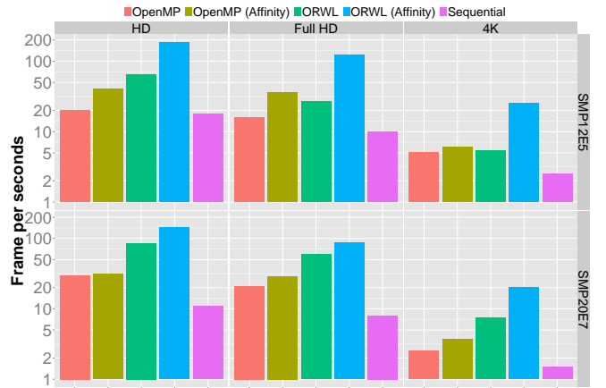
Figure 6. FPS (logarithmic scale) of HD video tracking
