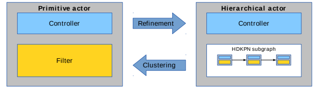
Fig. 3. Refinement and clustering between a primitive actor and its corresponding hierarchical actor.
