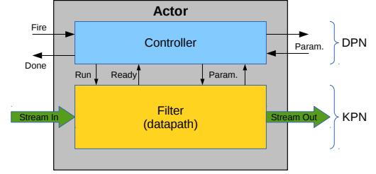
Fig. 2. Decomposition of a DKPN actor into its controller and its filter. The controller exchanges commands ( fire/done ) with the scheduler and parameters with other actors. It drives the filter through run and ready commands and reconfigures it through internal parameters. The filter exchanges data with other actors via streaming interfaces and processes them. Controller and filter respectively belong to DPN and KPN spaces.
