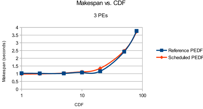
Fig. 6. Comparison of execution times of the TNR application in reference and scheduled PEDF with different variability levels for overhead evaluation.
