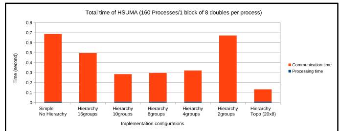
Figure 12: Comparison of execution time of simple, topology-oblivious hierarchical and topological implementations on NTW10E5. 160 processes process 1 block of 8 doubles
