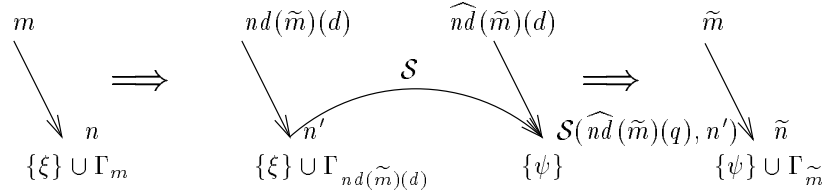
Figure 11: Finding \tilde{n} for n .
