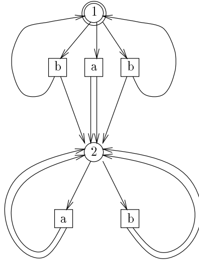
Figure 2: Tree automaton
