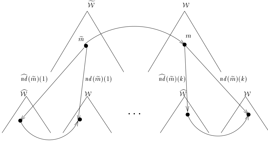
Figure 10: Auxiliary functions
