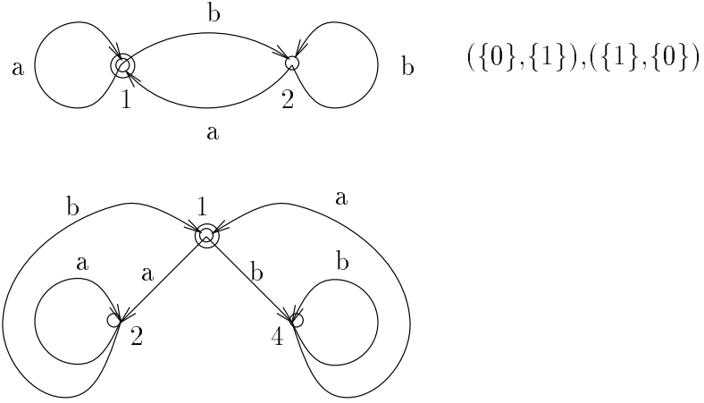
Figure 1: An automaton for \{w \in \{a, b\}^* : |w|_a < \infty \text{ or } |w|_b < \infty\}
