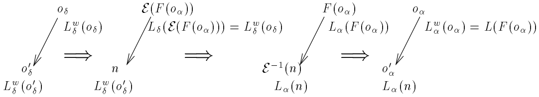
Figure 8: Finding a \langle a \rangle -son of o_\alpha for a \langle a \rangle -son of o_\delta .
