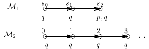
Figure 3: Models \mathcal{M}_1 and \mathcal{M}_2
