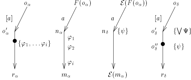
Figure 9: Finding r_\delta for r_\alpha .
