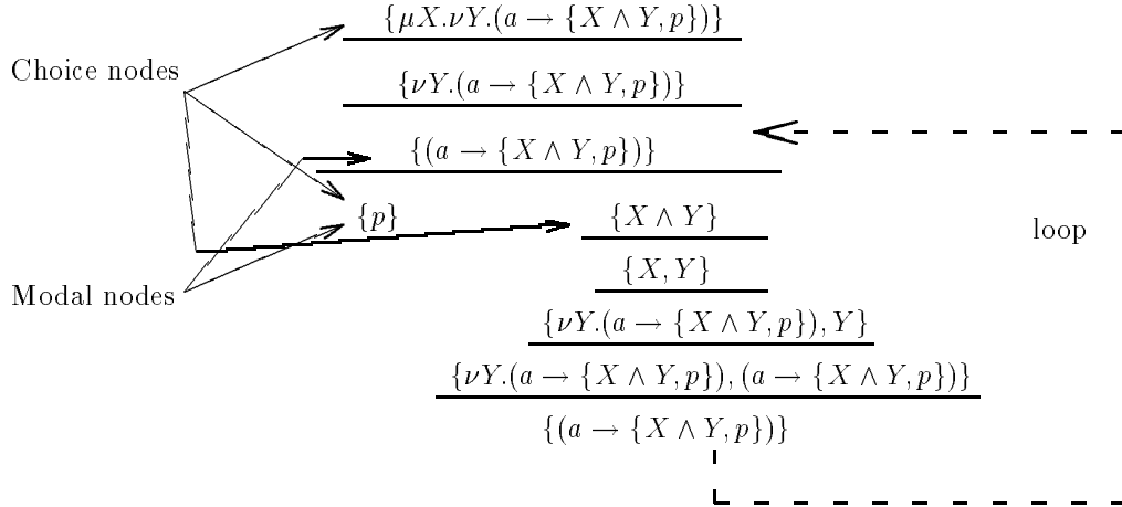
Figure 5: An example of a tableau.
