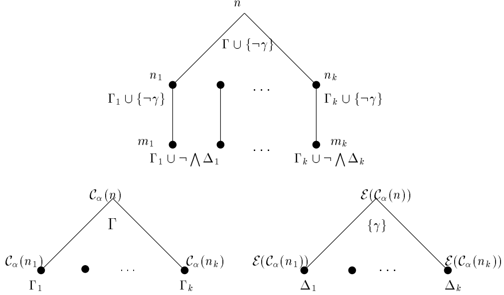
Figure 7: The proof of Observation 9.2.1. The labels of the nodes are written below the nodes.
