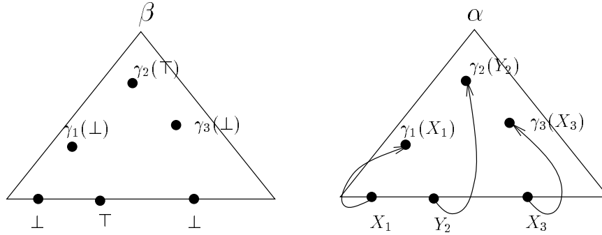
Figure 6: Tableaux \mathcal{T}_\beta and \mathcal{T}_\alpha
