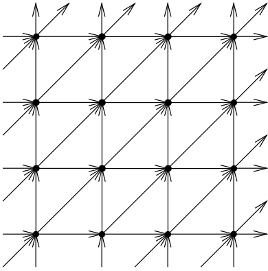
Figure 2: A portion of H
