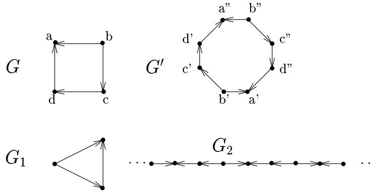
Figure 1: Example of d1-covering
