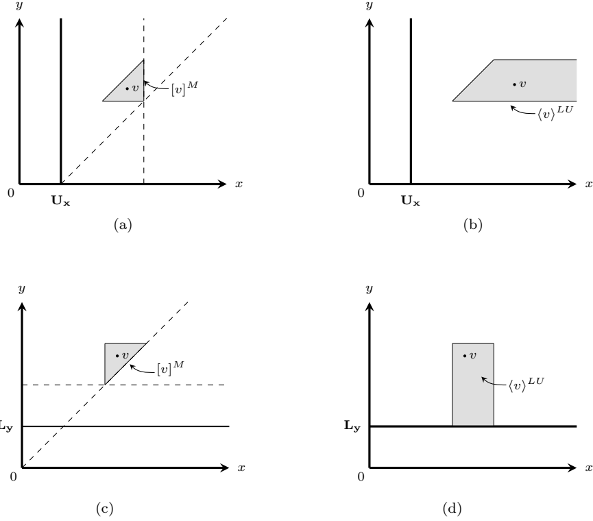
Figure 7: \langle v \rangle^{LU} can be thought of as a transformation of [v]^M by altering select constraints. Pictures (a) and (b) handle the case when v_x > U_x ; pictures (c) and (d) handle the case when v_y > L_y
