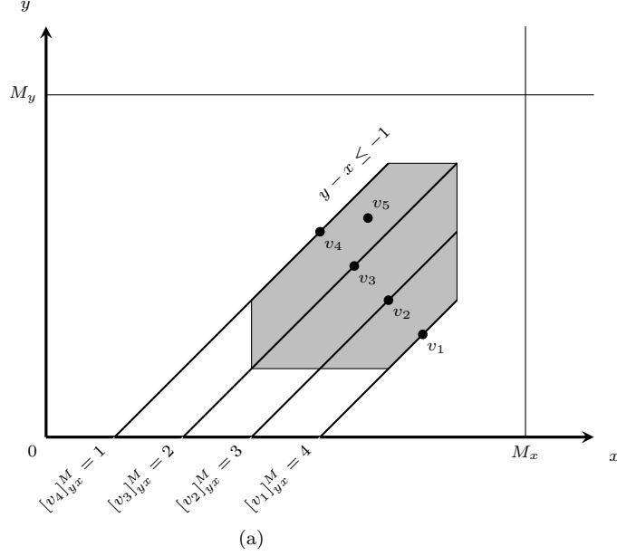
Figure 9: Value of [v]_{yx}^M decreases as we move left
