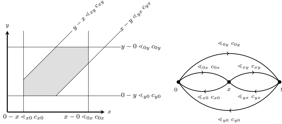
Figure 6: An arbitrary zone with its constraints and distance graph
