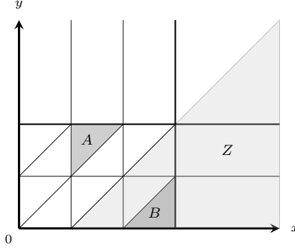
Figure 8: A bounded region is either totally contained in a zone Z or totally disjoint from it. It can never intersect partially. For example, the bounded region B is totally inside Z , however the bounded region A is totally disjoint from Z .
