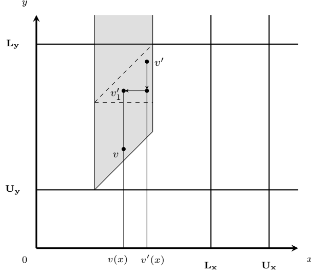
Figure 4: Intuition for the adjustment lemma.
