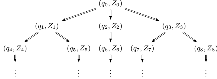
Figure 5: A reachability tree of zones computed by a forward exploration
