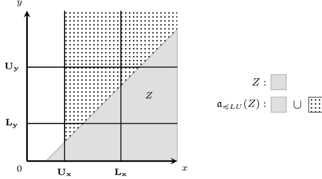
Figure 3: Zone Z is given by the grey area. Abstraction \mathbf{a}_{\preceq LU}(Z) is given by the grey area along with the dotted area
