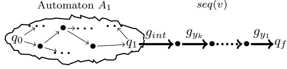
Figure 2: Adding the sequence seq(v) to A_1 .
