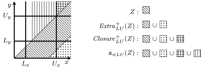
Figure 1: A comparison of abstraction operators for zones.
