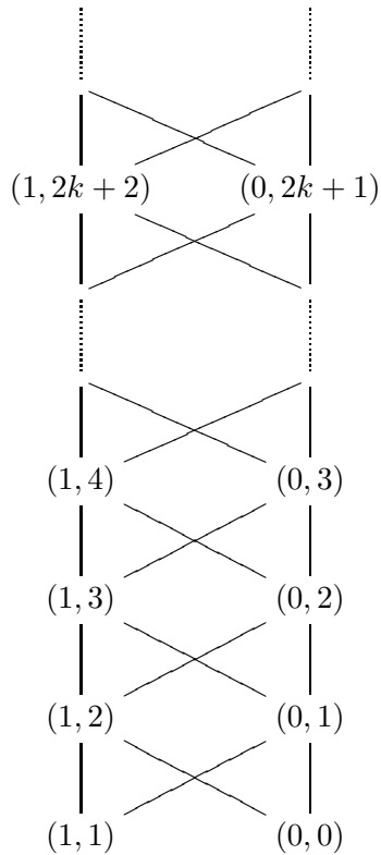
Figure 1: Hierarchy of Mostowski indices.
