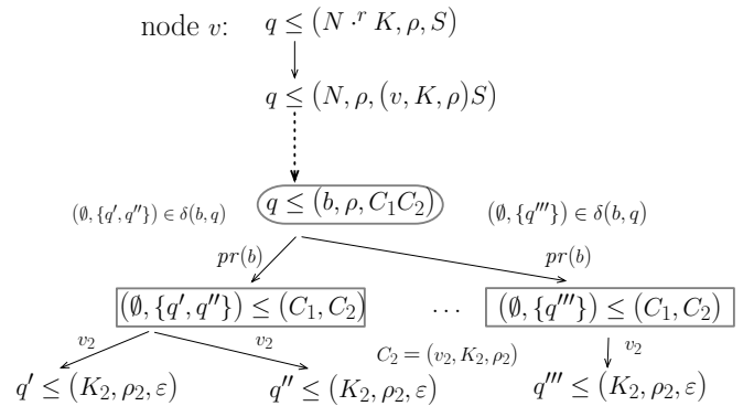
Fig. 4. Game K(M, \mathcal{D}, q_0) . Eve chooses in rounded boxes, and Adam in rectangular boxes.
