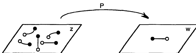
Fig. 2. Inverse image of a segment.
