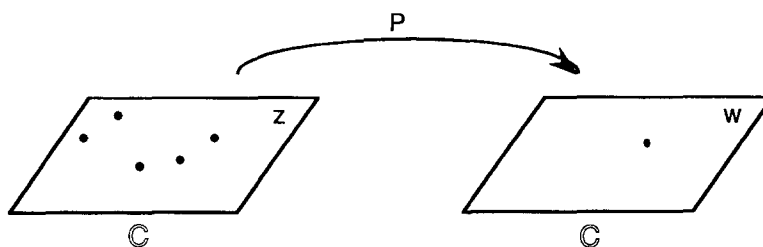
Fig. 1. Inverse image of a point.
