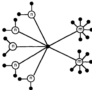
Fig. 10. One of the three plane trees of the type \langle m, m, n, n, n, n, n; 7, 1, \dots, 1 \rangle .
