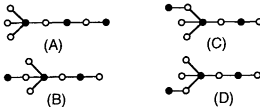
Fig. 9. Two orbits of Galois group.
