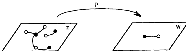
Fig. 3. Ends of some segments are critical points.
