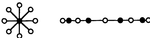
Fig. 4. Trees corresponding to z^n and T_n(z) .
