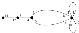
Figure 2: The “mouse map” with labelled half-edges
