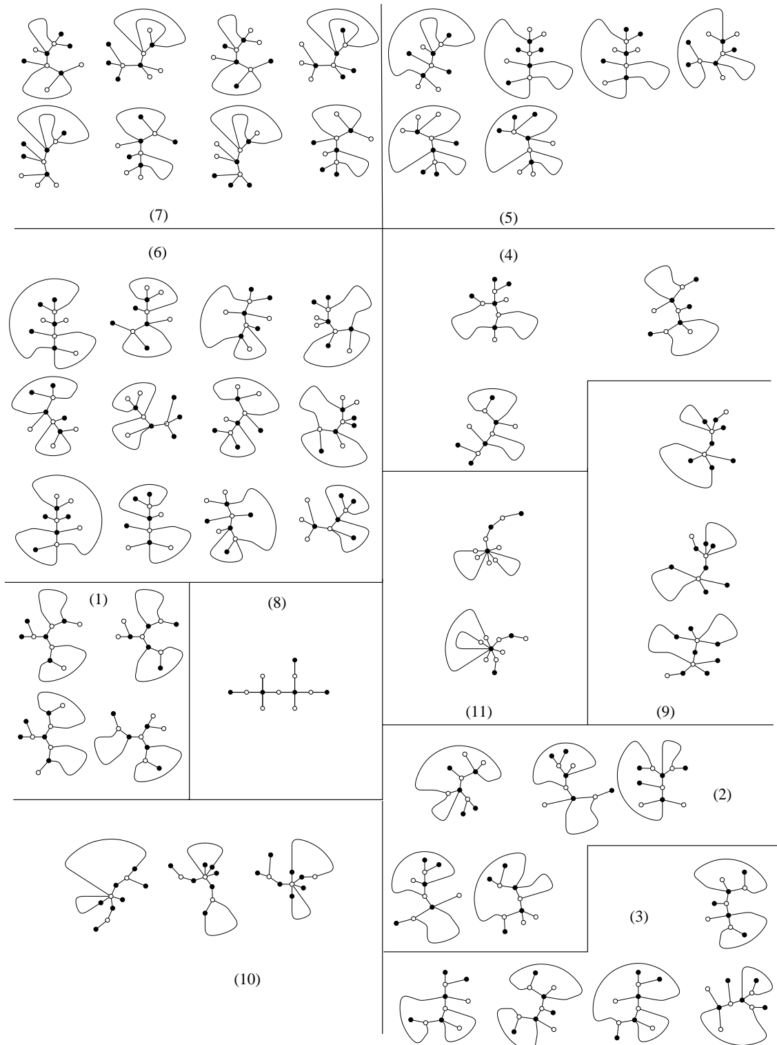
Figure 4: Planar hypermaps with cartographic group M_{11}
