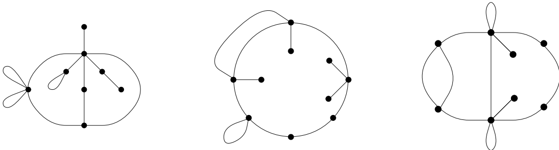
Figure 7: Three maps representing M_{24}
