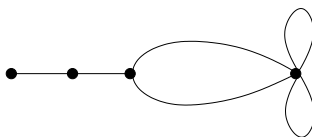
Figure 1: A planar map that represents the group M_{12}
