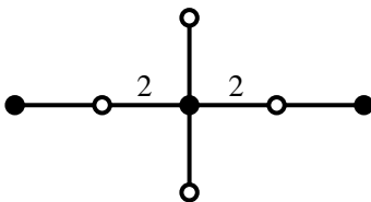
Figure 27: The symmetric tree with the passport (6^1 1^2, 3^2 1^2, 6^1 1^2) .
