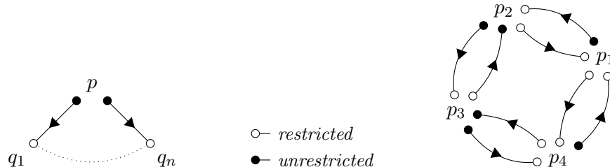
Figure 1: Examples of non-confluent typed topologies
