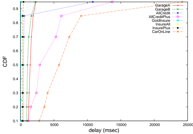
Figure 8. Empirical distribution of end-to-end orchestration delays for 100000 simulations in the bootstrapping case.
