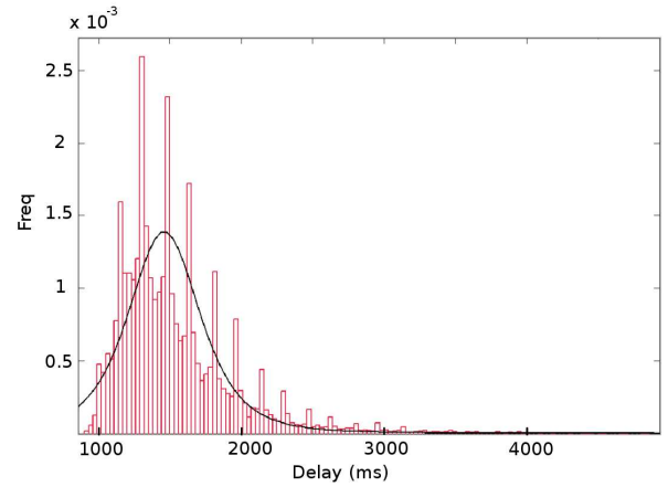
Figure 6. Fitting of a T Location-scale distribution on the plot of 20,000 measured delays of the service USWeather .
