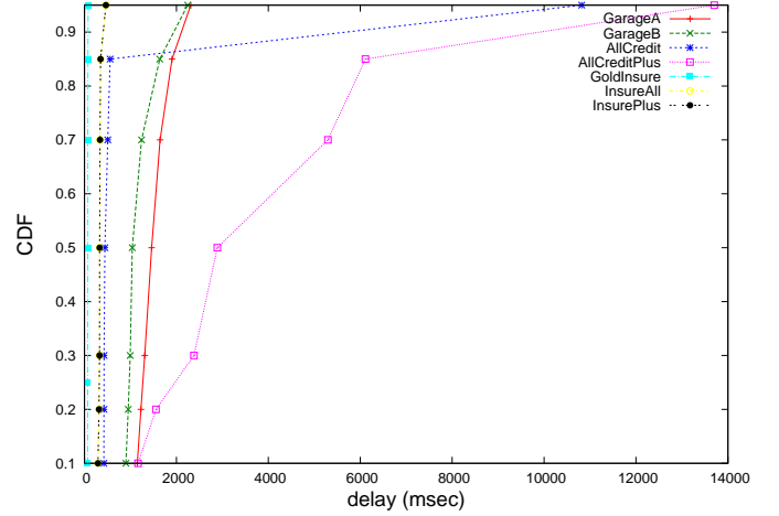
Figure 7. Cumulative distribution function for the measured delays of the six web services.
