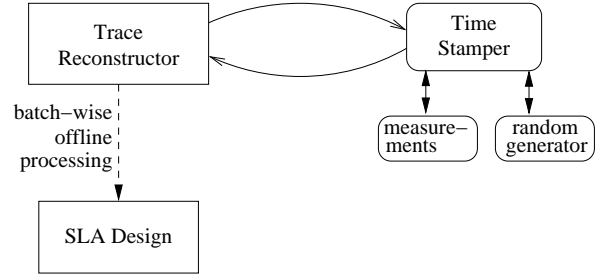
Figure 3. Overall architecture of the TORQuE tool.
