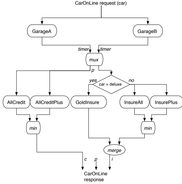
Figure 2. A simplified view of the CarOnLine orchestration. The calls to GarageA and GarageB are guarded by a timer that returns a “Fault” message whenever the timeout occurs—this is not shown on the figure. In the discussion in section II-B regarding “monotonicity”, the test car = deluxe is changed to p \geq limit .
