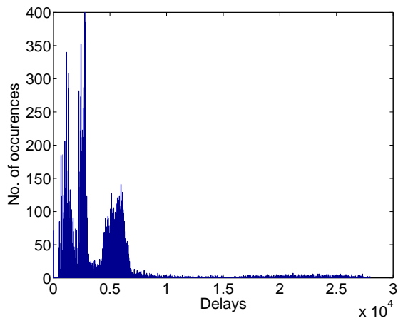
Figure 1. Measurement records for response times, for Web service StockQuote.
