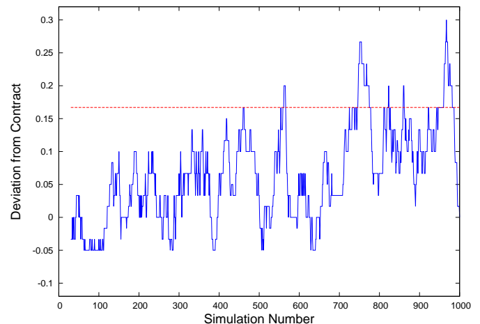
Figure 9. Monitoring of GarageA . The plot shows the deviation from its contract for each run of the simulation. This deviation is \sup_{x \in X} (F_S(x) - \hat{G}_{S, \Delta^*}(x)) .
