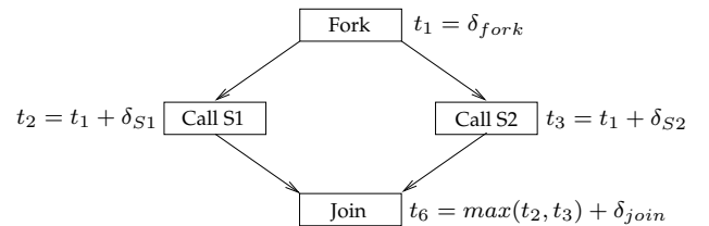
Figure 4. Deriving response time for a fork-join pattern. The “Fork” and “Join” are the branching and synchronization events, S1 and S2 are two web services called in parallel. \delta_a denotes the time taken for event a to execute.
