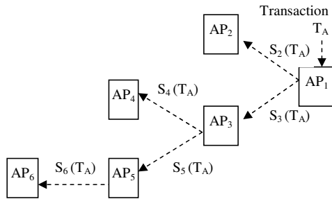
Figure 1. Nested recovery protocol for AXML recovery
