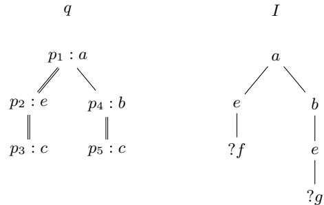
Figure 7: Example for hard relevance
