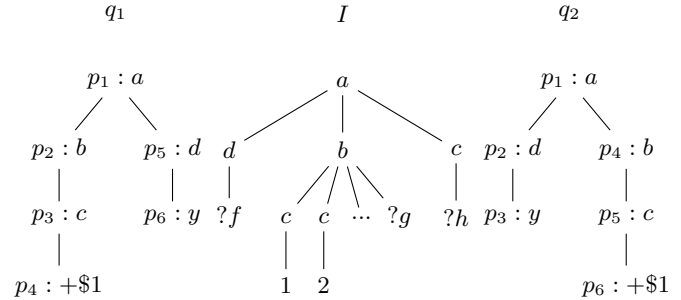
Figure 4: Beyond MagicSet
