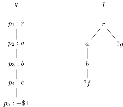
Figure 8: Example for nonmonotonic features
