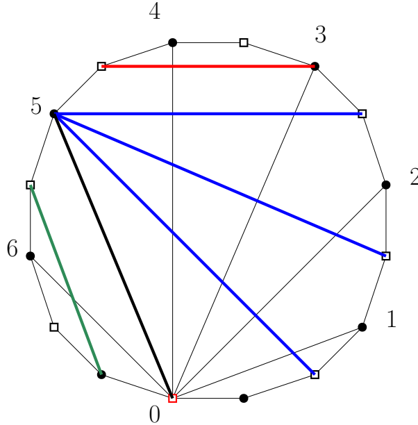
Figure 6: The quadrangulation Q associated to the monomial x_5 y_3^3 y_7 with P_Q = (x_5 - y_4)(y_5 - x_3)(y_5 - x_2)(y_5 - x_1)(y_7 - x_6) .
