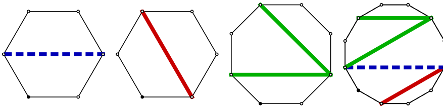
Figure 8: B_0, B_1, B_2 and G(B_0; B_1, B_2)
