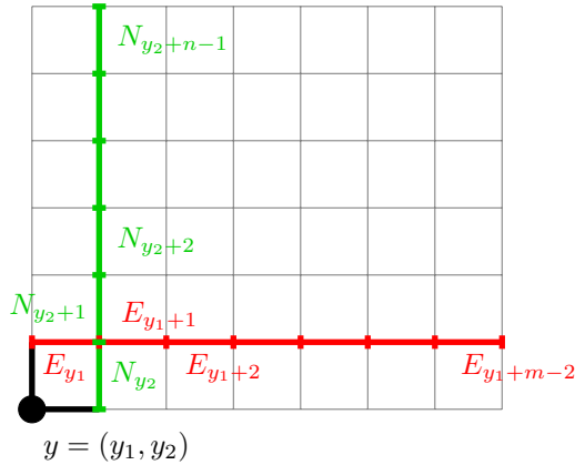
FIGURE 4. The frame \text{Frame}_{m,n}^y .
