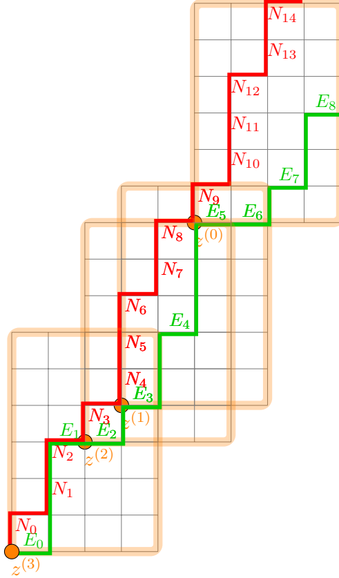
FIGURE 2. The relevant part of ((Nu'')^{\mathbb{Z}}, (E\ell')^{\mathbb{Z}}) to compute \pi(u'', \ell') and the iterations of \varphi^k(u) for binomials paths u'' = ENNENENN , \ell' = NNNEENENN and configuration c = \begin{pmatrix} 1,2,2,3,3,3, \\ 0,3,5,* \end{pmatrix} on K_{4,6} . The other pairs of binomial paths that stem from the stable intersections in the diagram are (u'', \ell') = (ENNNENNE, NENNNENNNE) , (NNENNENE, NNENNNEEN) , and (ENNNENNE, ENENNNENN) .
