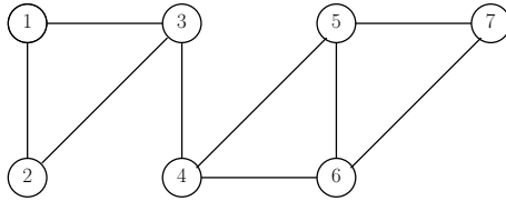
FIGURE 1. The graph G of Example 2.10.
