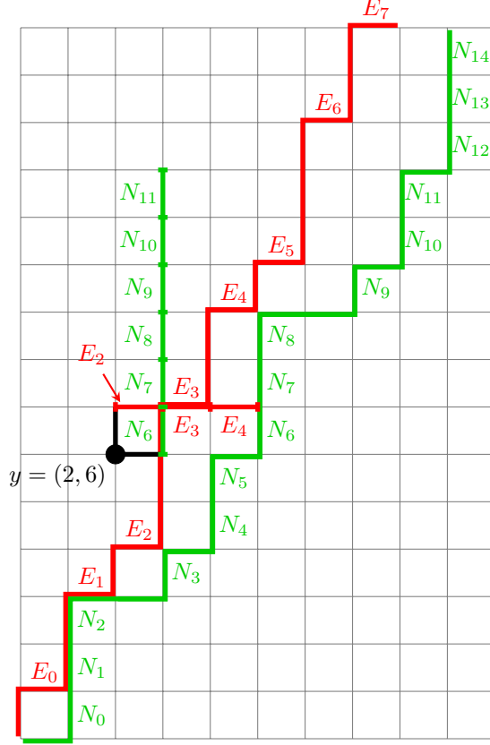
FIGURE 6. Example of moving the frame of Figure 5 one step south. Note that m = 4 and n = 6 .
