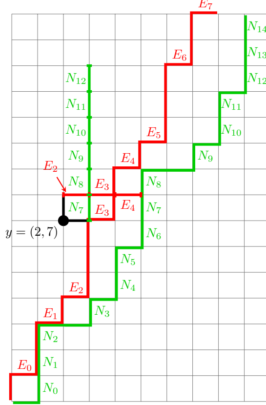
FIGURE 5. The frame and bi-infinite path of Example 5.3. Note here that m = 4 and n = 6 .
