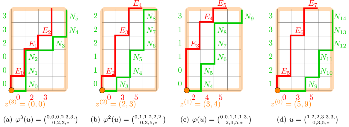
FIGURE 7. The toppling and permuting equivalent sorted stable configurations from parking to recurrent configurations. We remind the reader that \varphi^3 is a parking function.
