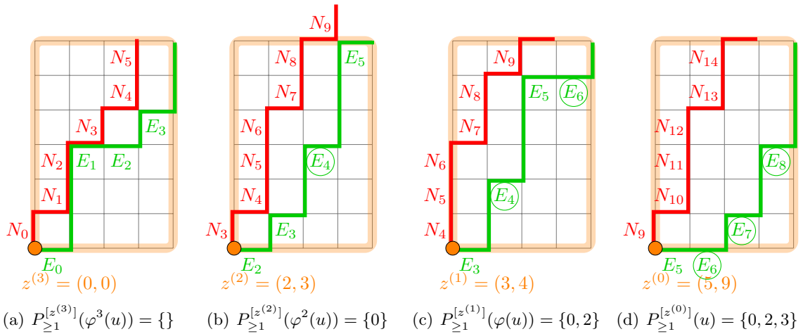
FIGURE 8. Evaluation of P_{\geq 1}^{[z^{(i)}]} from parking to recurrent configurations as in Figure 7.
