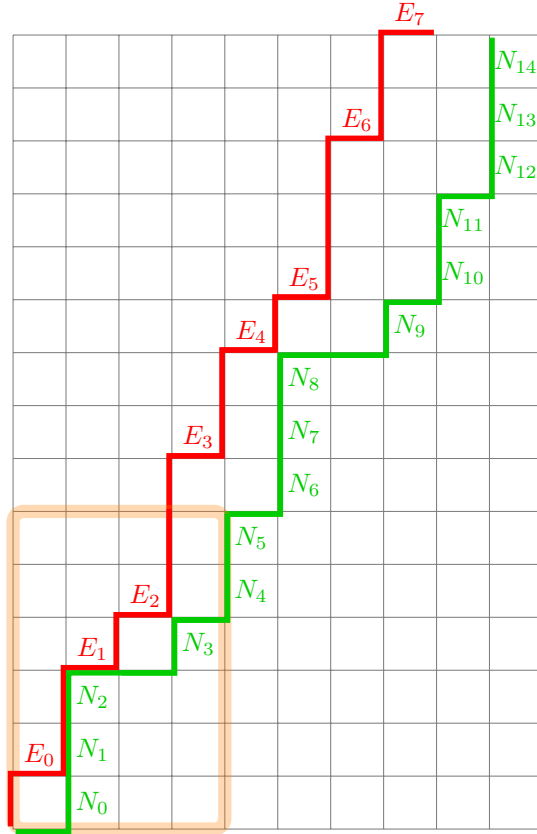
FIGURE 3. The NE labelling of the pair of bi-infinite paths ((Nu'')^{\mathbb{Z}}, (E\ell')^{\mathbb{Z}}) where u'' = ENNENENN , \ell' = NNNEENENN . The bottom left corner is the origin. Notice that the steps that have been labelled are precisely those steps of Figure 2 that were not labelled. Note that m = 4 and n = 6 .
