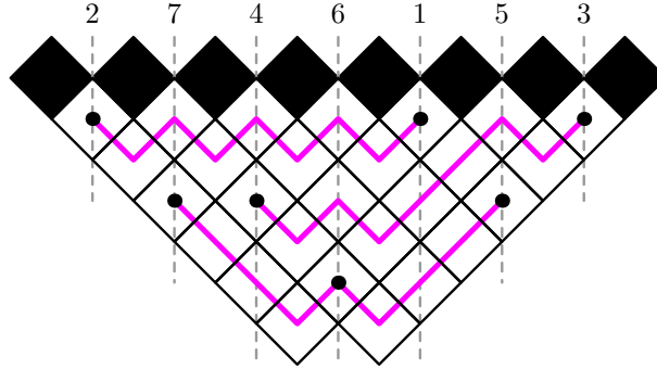
Figure 18: The ribbons represent the patterns 2^+2 in the permutation
