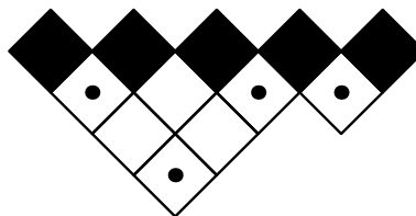
Figure 8: A Dyck tableau and its basement
