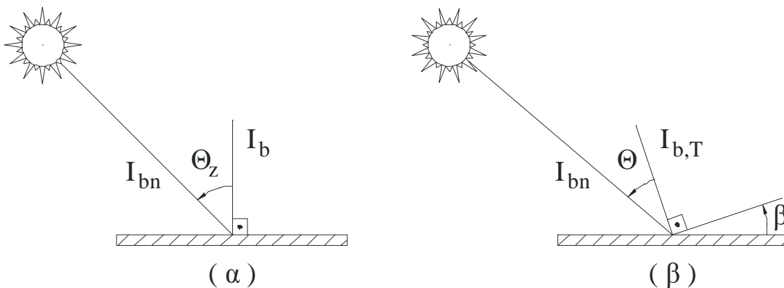
Figure 4.2 Determination of conversion factors for the direct solar irradiance. α) Irradiance on horizontal surface β) Irradiance on inclined surface
