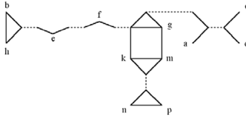
Figure 2: The split decomposition of G .
