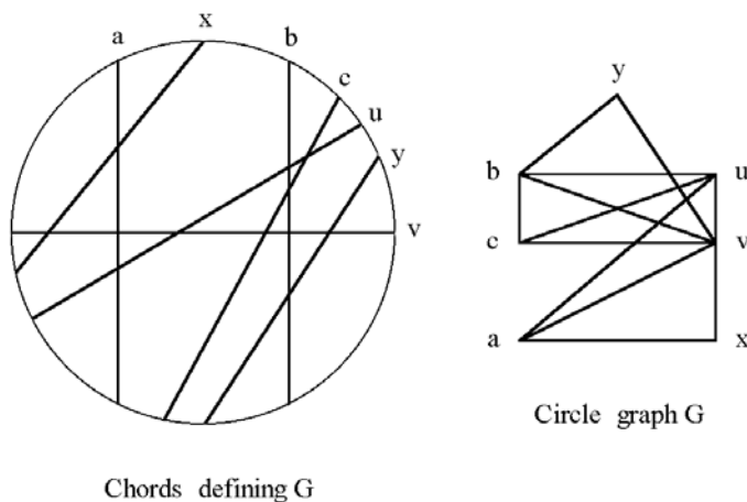
Figure 3: A circle graph and a chord representation of it
