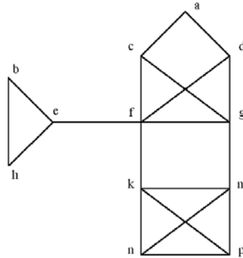
Figure 1: Graph G
