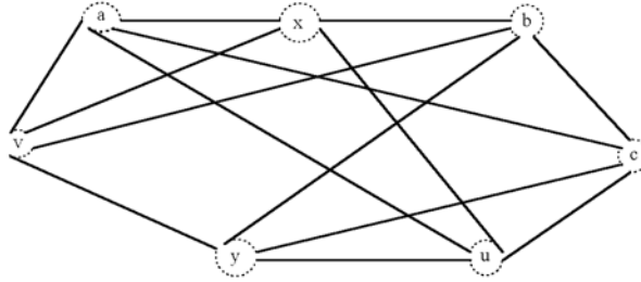
Figure 4: The neighbourhood graph N(G) .
