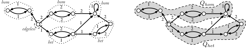
■ Figure 5 Example of G_A with the subgraphs induced by Q_{hom} and Q_{het} . For simplicity we assume that \mathbb{A} = \{a\} and we hence omit the letter a when depicting edges labeled by (i, a) .
