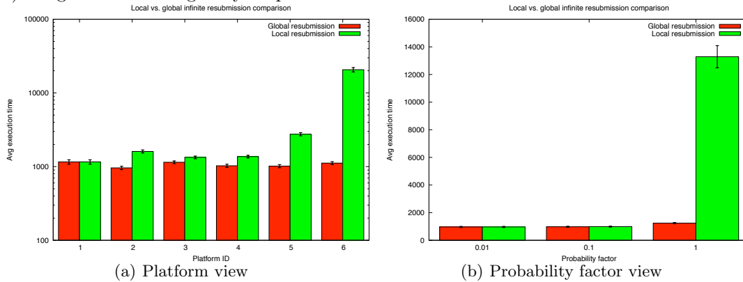
Fig. 2. Comparison of the unlimited local vs. global resubmission
