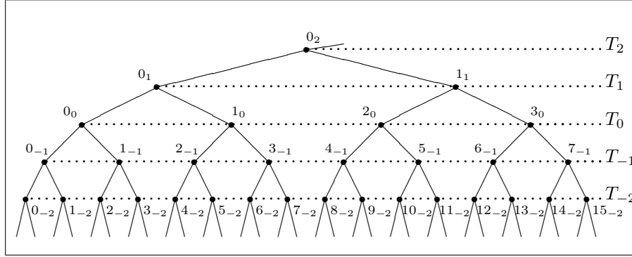
Figure 3. The 2-refinable totally unbounded layered structure
