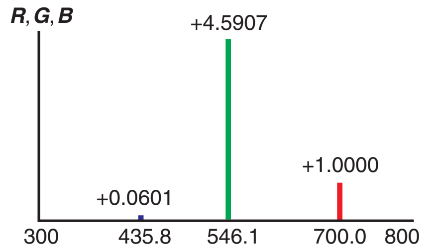
CIE primaries \mathbf{R}, \mathbf{G}, \mathbf{B}
