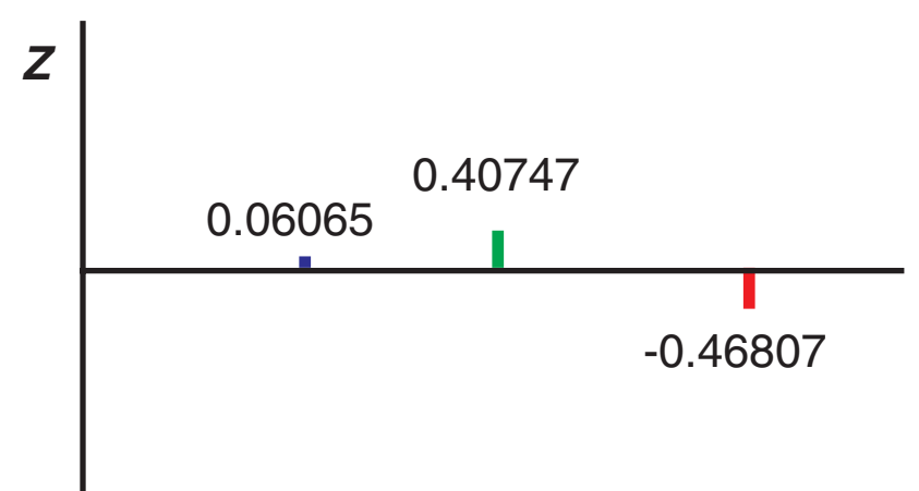
Synthetic primaries \mathbf{X}, \mathbf{Y}, \mathbf{Z}
