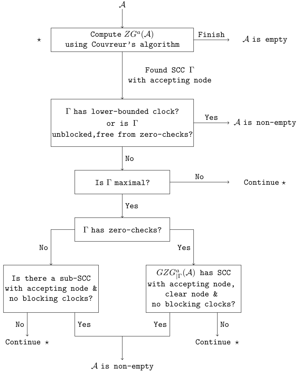
Figure 10: Algorithm to check for Büchi emptiness of \mathcal{A} . “Continue” loops back to computing ZG^a(\mathcal{A}) using Couvreur’s Algorithm.
