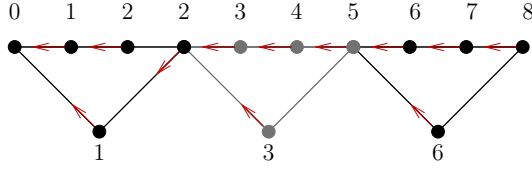
Fig. 4. Configuration X_1 of \mathcal{G}_3
