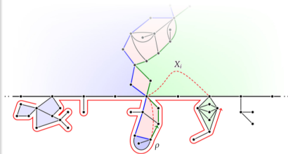
UIHPQ (sketch by N. Curien & A. Caraceni).
