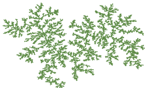
Uniform random tree 50k edges.
