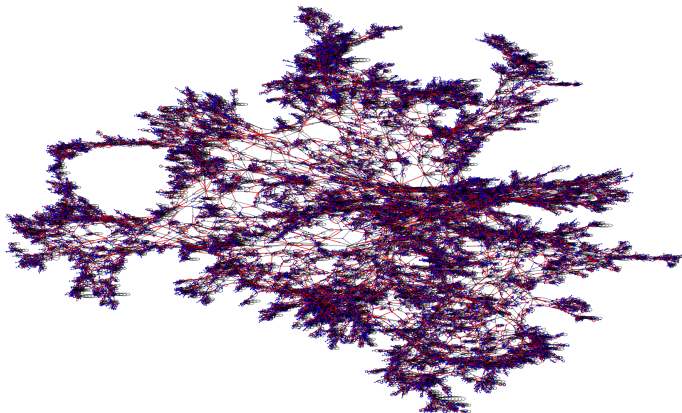
Uniform ST map 100k edges.
