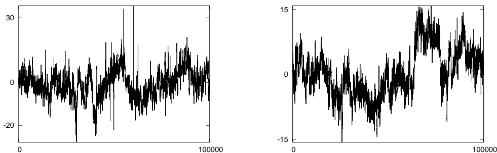
Figure 7: Simulations of R_n associated with a plane tree with 50000 nodes, where Y is symmetric and satisfies \mathbb{P}(|Y| > y) = (1 + y)^{-a} for y non-negative and a = 3 for the first figure and a = 4 for the second one.
