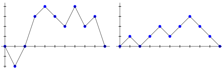
Figure 3: Interpolation of processes R_n and V_n associated with the marked tree of Figure 1
