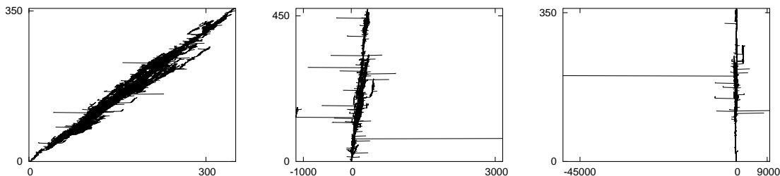
Figure 9: Discrete branching random walk (size 100 000) with values 1+y where Y is symmetric and satisfies \mathbb{P}(|Y| > y) = (1+y)^{-5/2} for y \geq 0 , \mathbb{P}(|Y| > y) = (1+y)^{-3/2} for y \geq 0 , and for the last one \mathbb{P}(|Y| > y) = (1+y)^{-1.1} for y \geq 0 .
