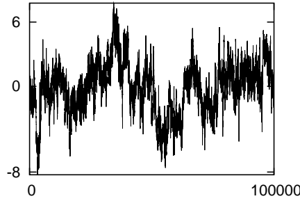
Figure 5: Simulation of R_n associated with a random plane tree with 50000 nodes, where Y is symmetric and satisfies \mathbb{P}(|Y| > y) = (1 + y)^{-6} for y non-negative.
