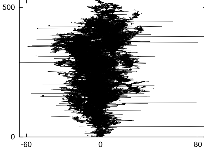
Figure 8: Discrete branching random walk (size 150 000) where Y is symmetric and satisfies \mathbb{P}(|Y| > y) = (1 + y)^{-5/2} for y \geq 0 .
