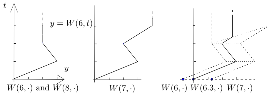
Figure 4: Three stopped paths associated with the BRW of Figure 1.
