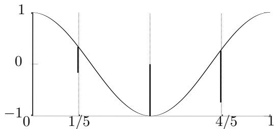
Figure 6: Representation of H(f, \Xi) with f(x) = \cos(2\pi x) and \Xi = \{(\frac{1}{5}, -\frac{1}{2}), (\frac{1}{2}, 1), (\frac{4}{5}, -1)\}
