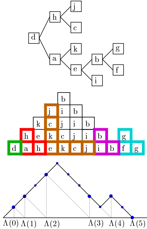
Figure 3.1 : Excursion - Binary tree
