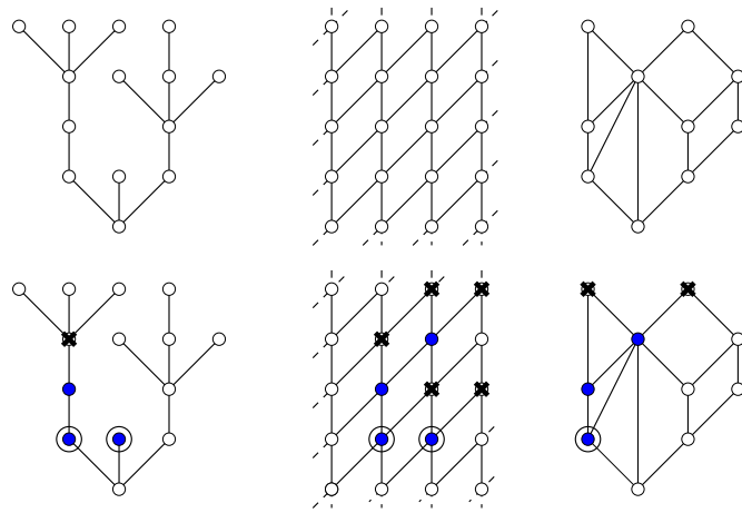
Figure 1: On the first line, three examples of agreeable graphs on which the directed edges are directed upwards. The first example is a tree, the second is the square lattice and the third a “non-layered” agreeable graph. On the second line are represented some DA on these graphs; filled points are the cells, the crosses are perimeter sites, and the surrounded points are the minimal sources of these DA.
