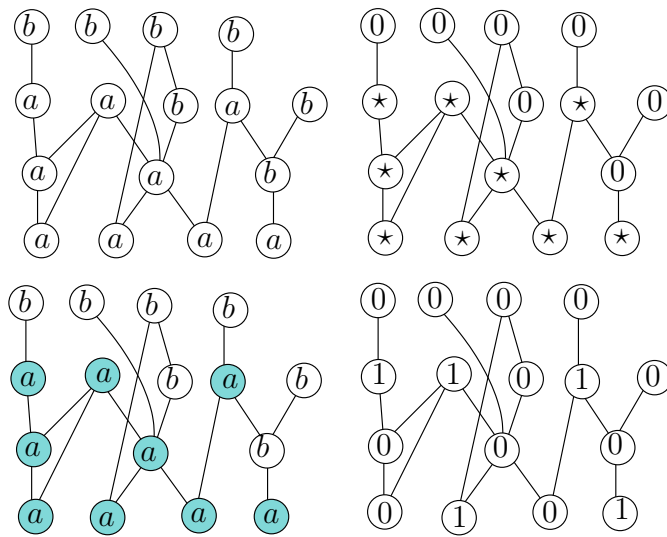
Figure 3: On the first column on top, a random coloring. Below, the family of DA derived from it. On the second column on top, the beginning of the computation of the gas occupation. “*” stands for the places where the calculus X_x \leftarrow \prod_{c: \text{children of } x} (1 - X_c) must be done. Below, the gas occupation has been computed.
