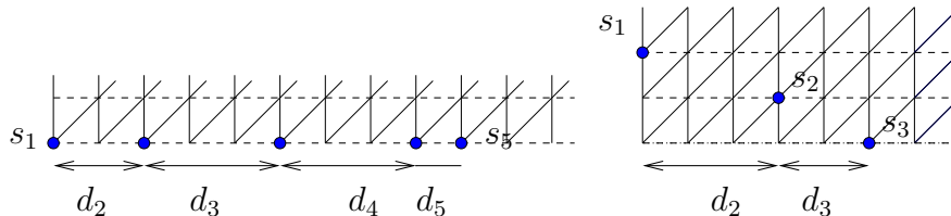
Figure 9: On the first picture, the sources considered in Proposition 3.6. The second picture illustrates the sources considered in Proposition 3.7.
