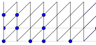
Figure 12: A DA on the cylinder. The maximum source has 4 cells, the area is 10. The right most and left most vertices are identified.
