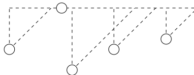
Figure 10: The points stands for the points of S ; the dotted lines surround the (finite) set of cells where the summation has to be done.
