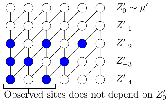
Figure 7: The colored sites are the sites where the Bernoulli( p ) coloring = 1. The gas occupation on the three first cells on the last row depends only on the DA (with these three cells as over-sources). The height of this DA is so small that the gas occupation of these cells does no depend on Z'_0 .
