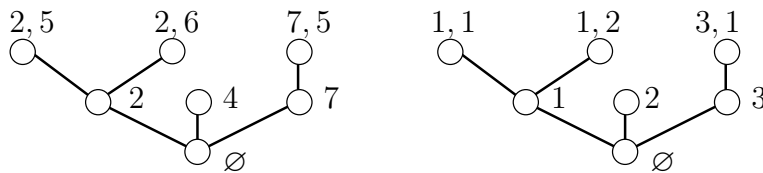
Figure 4: The trees admit some usual representation as embedded figure in the plane, mapping the order between brothers into the usual order between the abscissas. In the usual Neveu's convention, there is an additional axiom (if v = u_1 \dots u_k j \in \mathbf{t} for some j \geq 2 then v = u_1 \dots u_k(j-1) \in \mathbf{t} ) which ensures that the "branching structure of the tree" characterizes the tree (for Neveu, only the second drawing represents a tree). This is not the case, here.
