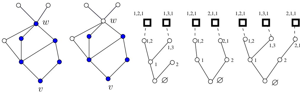
Figure 6: On the first picture, a DA A^{\{v\}} (whose cells are colored). On the second one, a DA A' obtained from A^{\{v\}} by the suppression of a cell having no child. The three trees with straight lines represent trees embeddable in A' at v . The trees with in addition some of the dotted lines are the trees embeddable in A^{\{v\}} at v . The square nodes are the nodes whose embedding are w
