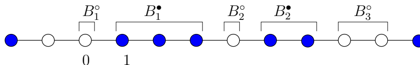
Figure 8: On this example, the black cells are occupied and corresponds to the places where Z = 1 , and the whites one are empty.
