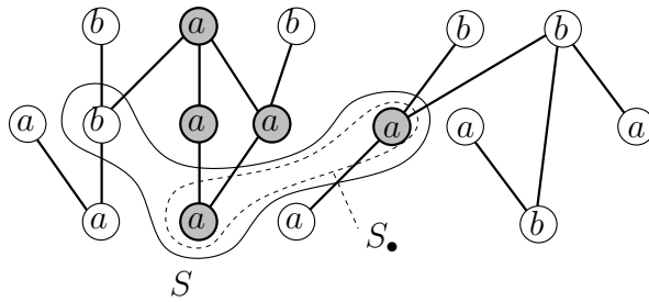
Figure 2: The DA \mathbf{A}^S(\omega) is the set of gray cells.
