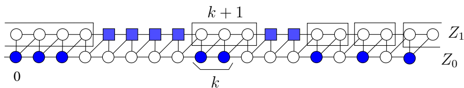
Figure 11: A block of k occupied positions in Z_0 determines k + 1 empty position on Z_1 (surrounded by rectangles). The little squares figure out the uncertain cells, that can not be determined just in view of the gas occupation in Z_0 .
