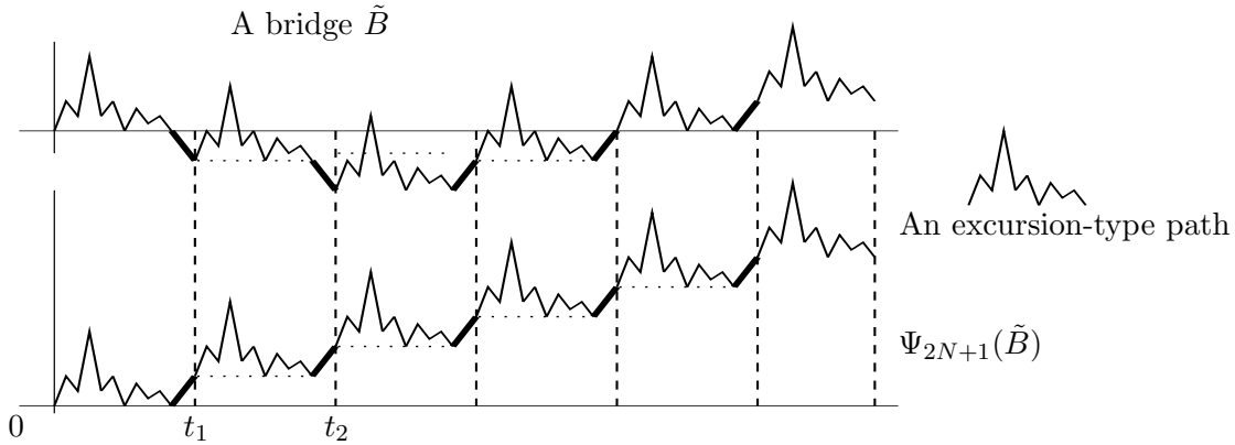
Figure 7: Synthetic description of \Psi_{2N+1} . The map \Psi_{2N+1} turns over each increment corresponding to a reaching time of a negative position. The map \Psi_{2N+1}^{-1} turns over the last increments reaching each position x \in \llbracket 1, \lfloor Z_{2N+1}/2 \rfloor \rrbracket ( Z_{2N+1} is odd).
