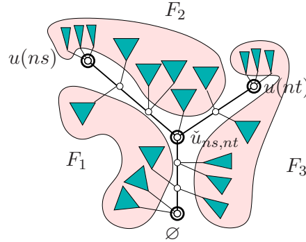
Figure 14: On this example w_1 = 321 , w_2 = 12 , w_3 = 2 , l = 1 , r = 3 , S_1 = 4 , S_2 = 8 , S_3 = 7 .
