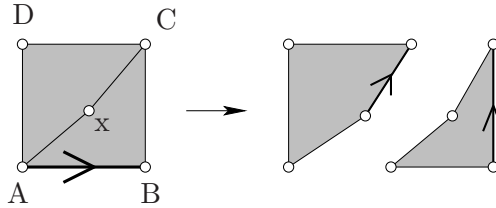
Figure 11: The decomposition is well defined thanks to the uniqueness of a node x adjacent to both A and C .
