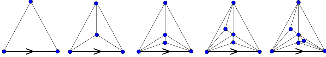
Figure 1: Iterative construction of a stack-triangulation. Note that three different histories lead to the final triangulation.
