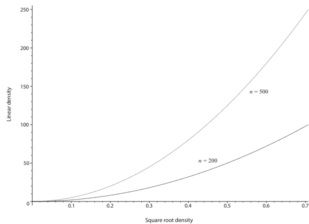
Figure 4: The curve shows how the “linear density” d_\ell (Eq. (1)) relates to the “square root” density d (Eq. (2)).
