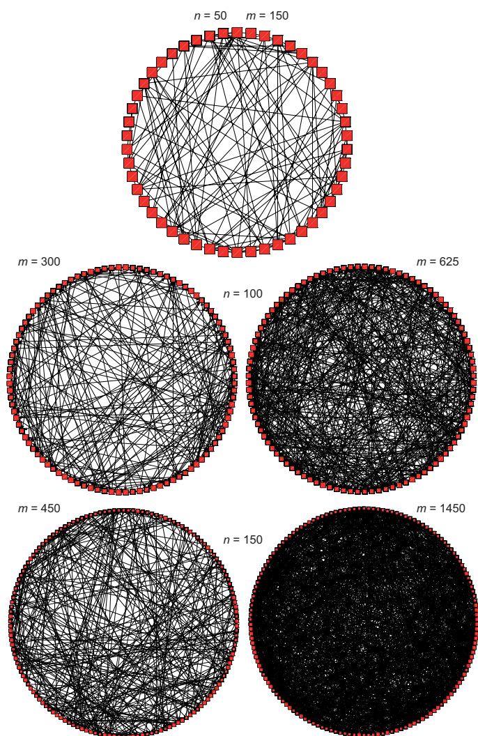
Figure 2: The picture gives a visual impression of how density d_\ell (left) and density d increase as n grows. We use fixed density d_\ell = 3 and d = 0.25 , so that the number of edges coincide for n = 50 .
