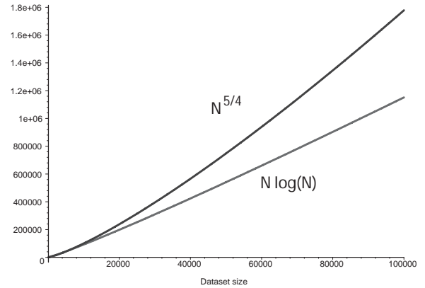
FIGURE 3.1: Comparison of the N^{5/4} and N \log N curves on the scale 10^3 - 10^6 .
