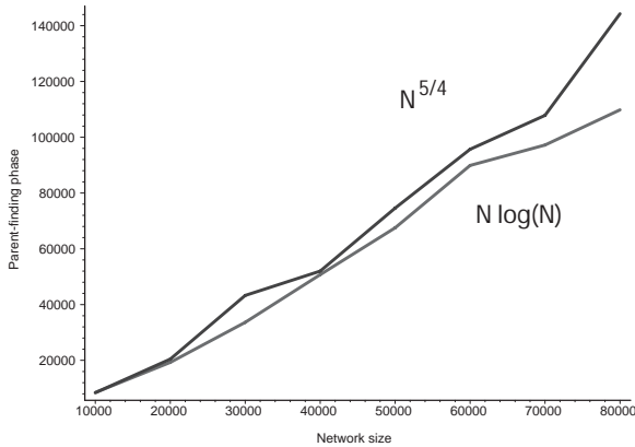
FIGURE 3.3: Comparing the actual time spent on the parent-finding phase.
