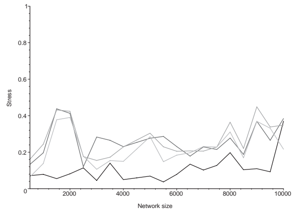
FIGURE 4.1: Comparison of Stress for all four MDS algorithms considered here. The darker curve at the bottom reports Stress values reached by the multiscale MDS.
