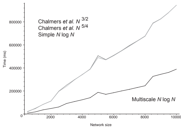
FIGURE 4.2: Comparison of the actual running time for all four MDS algorithms considered here.
