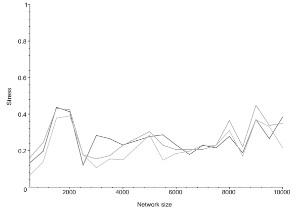
FIGURE 3.4: Comparison of Stress for the O(N^{3/2}) , O(N^{5/4}) (grayed) and the O(N \log N) (darker) MDS strategies.
