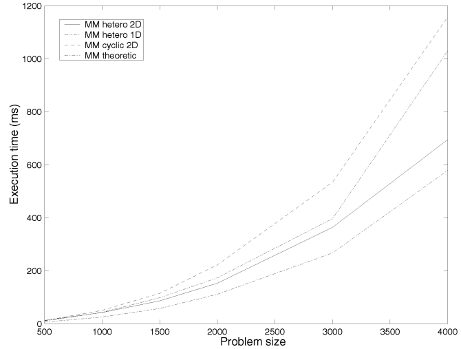
Fig. 16. Comparison of different allocations for matrix multiplication using nine processors.
