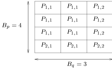
Fig. 6. A block panel with B_p = 4 and B_q = 3 for a 2 \times 2 processors grid of respective cycle-time t_{1,1} = 1 , t_{1,2} = 2 , t_{2,1} = 3 , and t_{2,2} = 6 . The processor P_{1,1} is twice as fast as the processor P_{1,2} , hence, it is assigned twice as many blocks within each panel.
