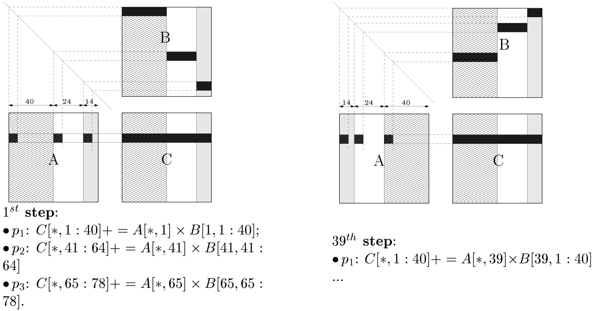
Fig. 2. Different steps of matrix multiplication on a platform made of three heterogeneous processors of respective cycle-times t_1 = 3 , t_2 = 5 , and t_3 = 8 . All indices in the figure are block numbers.
