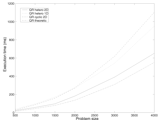
Fig. 17. Comparison of different allocations for QR decomposition using nine processors.
