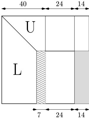
Fig. 3. Thirty-third step of LU decomposition (indices are block numbers): with the former distribution, the computation becomes less balanced. Here, after factoring block 33, processor 1 has seven updates and works for 7 \times 3 = 21 units of time, while processor 2 works 24 \times 5 = 120 units of time.
