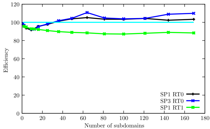
Fig. 7. Efficiency with SP1/SP3 equations and RT0/RT1 finite element.
