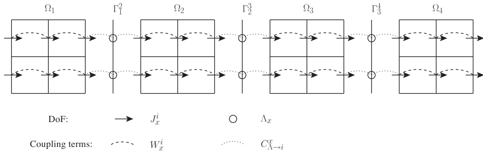
Fig. 3. \Omega is partitioned in N = 4 subdomains into the direction x . As we are interested in solving by domain decomposition the problem in the direction x after flux elimination, the flux \phi_i , the current J_i^j , the coupling terms B_i^d and A_i^j are ignored.
