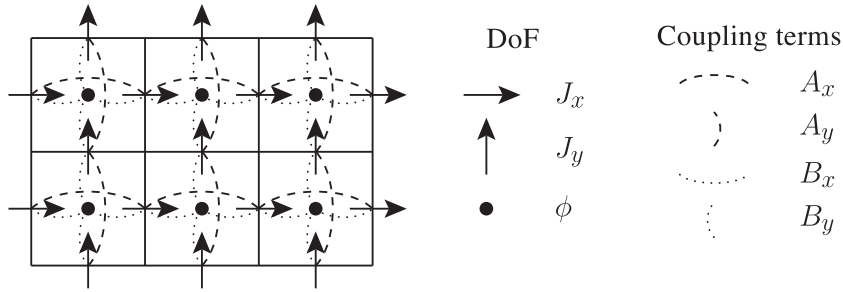
Fig. 1. Mesh, degrees of freedom (DoF) and coupling terms with the RT0 finite element for a 2D case.
