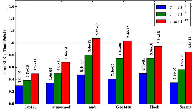
(a) Just-In-Time scenario using RRQR.
