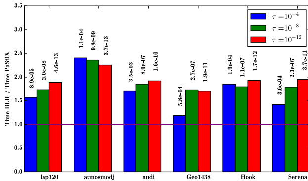
(b) Minimal Memory scenario using RRQR.
