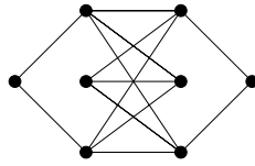
Figure 2.19: A graph G with mad(G) = \frac{13}{4} such that \chi_a(G) = \chi_a^l(G) = 5 .
