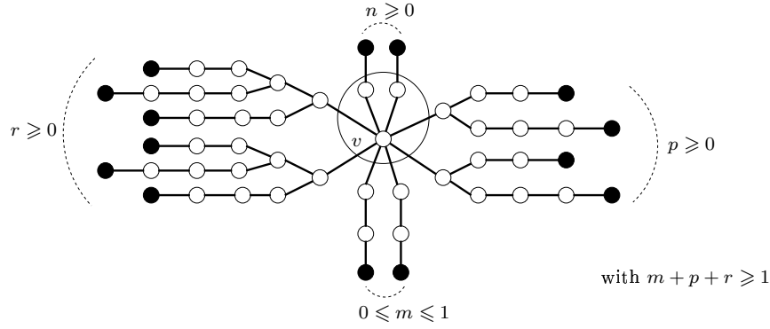
Figure 3.4: Forbidden configuration for Lemma 3.5.
