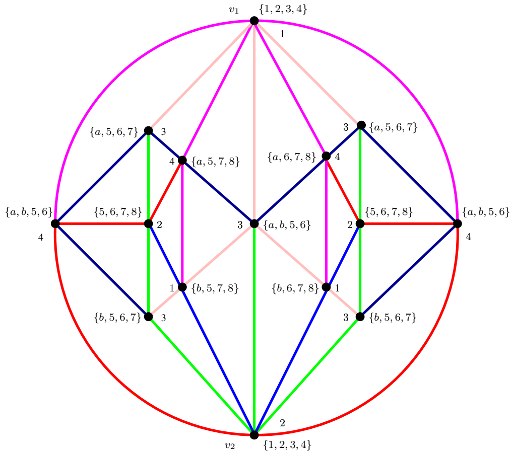
Figure 4.10: The forcing gadget F_{a,b} : 4-list assignment and acyclic 4-coloring.
