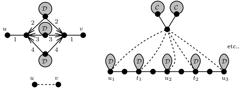
Figure 4.19: The vertex gadget for the reduction of Theorem 4.7.(6).
