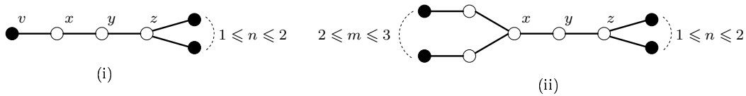
Figure 3.3: Forbidden configurations for Lemma 3.3.
