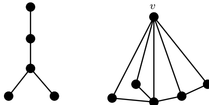
Figure 3.5: The tree T and the graph H_T .
