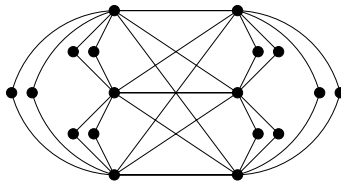
Figure 2.20: A graph G with mad(G) = \frac{11}{3} such that \chi_a(G) = \chi_a^l(G) = 6 .
