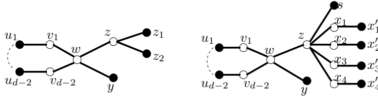
Figure 2.14: A d(d-2) -vertex adjacent to a weak vertex.
