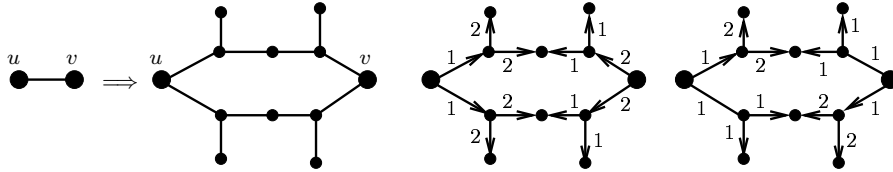
Figure 4.16: The edge gadget for the reduction for the reduction of Theorem 4.7.(4).
