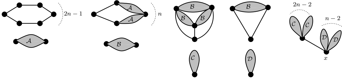
Figure 4.14: The vertex gadget for the reduction for the reduction of Theorem 4.7.(3).
