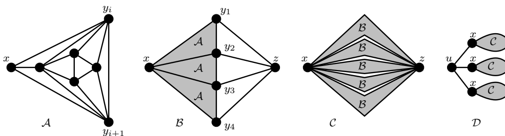
Figure 4.18: The forcing gadgets for the reduction of Theorem 4.7.(6).
