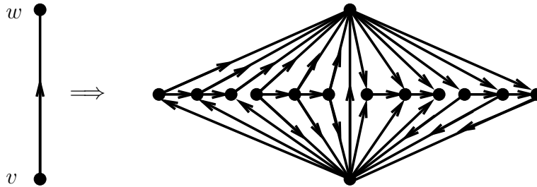
Figure 2.1: The graph we add to an arc.
