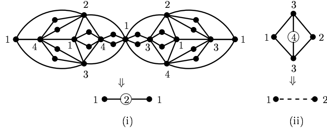
Figure 4.8: The forcing gadgets for the reduction of Theorem 4.5.
