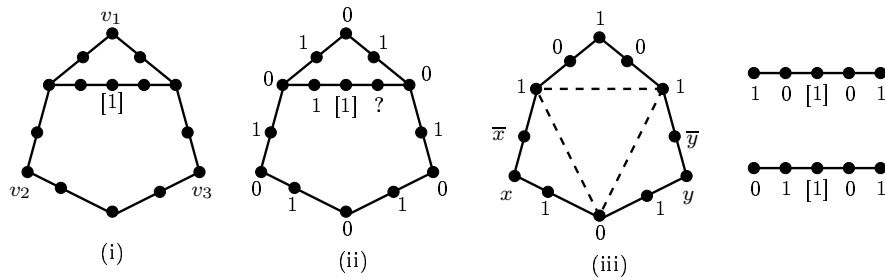
Figure 4.3: The clause gadget for the reduction of Theorems 4.1
