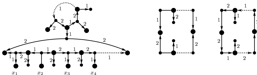
Figure 4.17: The vertex gadget and the edge gadget for the reduction of Theorem 4.7.(5).
