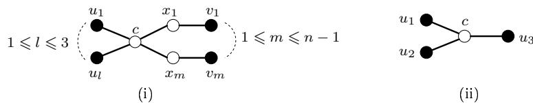
Figure 2.10: Forbidden configurations for Lemma 2.5.
