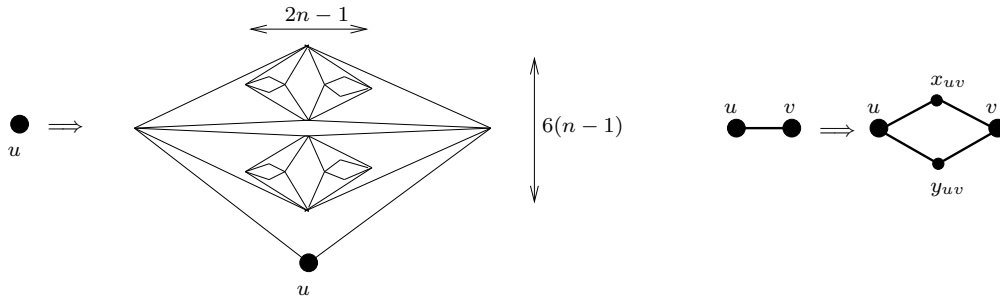
Figure 4.13: The vertex gadget and the edge gadget for the reduction of Theorem 4.7.(2).
