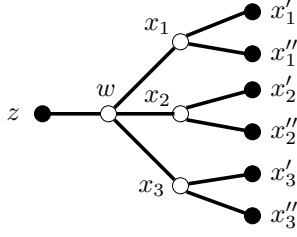
Figure 2.17: A 4-vertex adjacent to three 3-vertices
