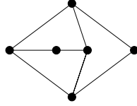
Figure 2.18: A graph G with mad(G) = \frac{8}{3} such that \chi_a(G) = \chi_a^l(G) = 4 .
