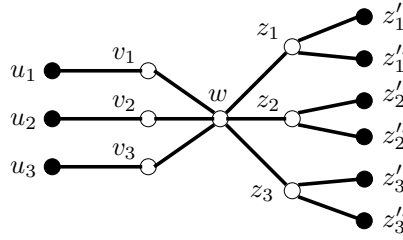
Figure 2.15: A 6(3)-vertex w adjacent to three 3-vertices.
