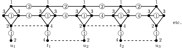
Figure 4.9: The vertex gadget for the reduction of Theorem 4.5.
