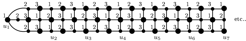
Figure 4.7: The vertex gadget for the reduction of Theorem 4.4.
