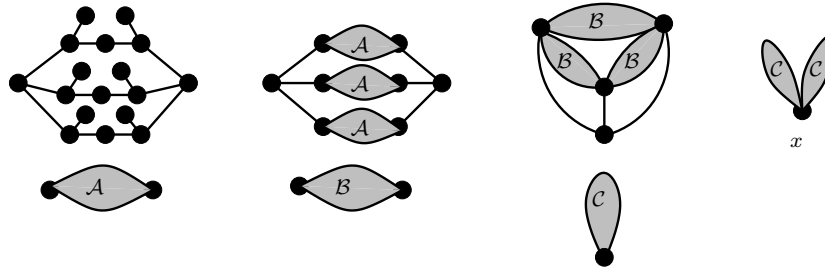
Figure 4.15: The vertex gadget for the reduction for the reduction of Theorem 4.7.(4).
