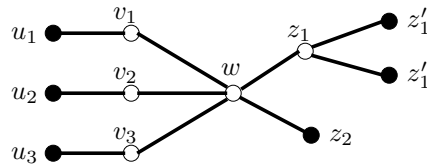
Figure 2.12: A 5(3)-vertex adjacent to a 3-vertex.
