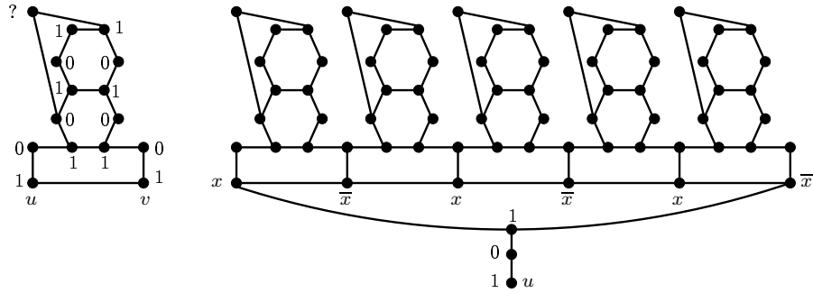
Figure 4.1: The forcing gadget for the reduction of Theorem 4.1.
