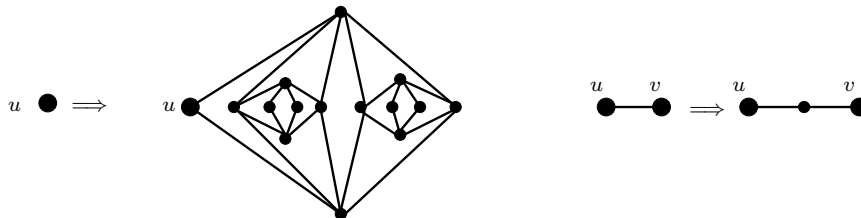
Figure 4.11: The vertex gadget and the edge gadget for the reduction of Theorem 4.7.(1).
