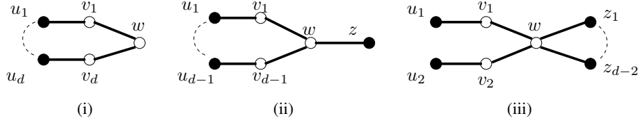
Figure 2.11: (i): A d(d) -vertex. (ii): A d(d-1) -vertex. (iii): A d(2) -vertex.
