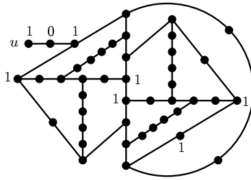
Figure 4.4: The forcing gadget for the reduction of Theorem 4.2.
