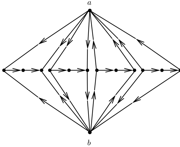
Figure 2.9: How to force a good pair in a target graph.
