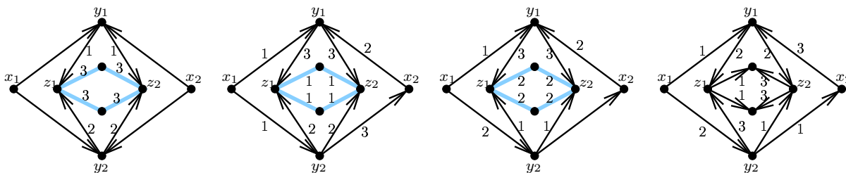
Figure 4.12: 3-P_4 -fa coloring with conditions on x_1 and x_2 .
