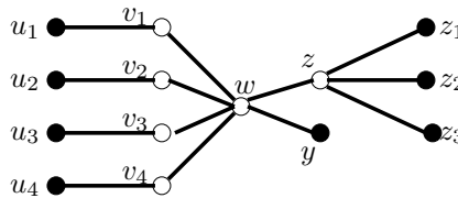
Figure 2.16: A 6(4)-vertex adjacent to a 4-vertex
