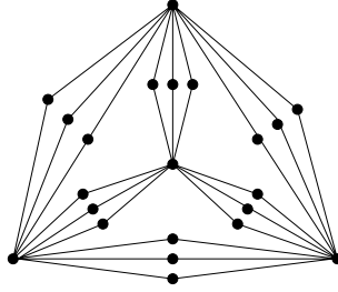
Figure 2.21: The graph G_n is such that mad(G_n) = 4 - \frac{8}{n^2+2} and \chi_a(G_n) = \chi_a^l(G_n) = n + 1 .
