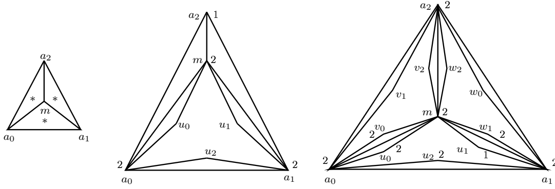
Figure 2.4: The graph G considered in Lemma 2.3.
