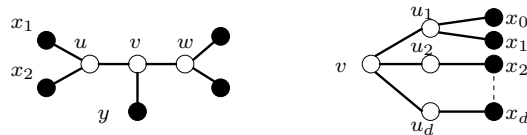
Figure 3.2: Forbidden configurations for Lemma 3.3.
