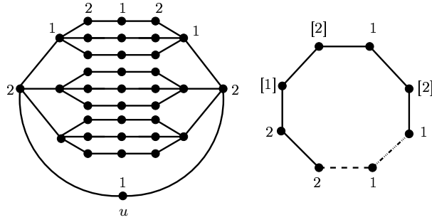
Figure 4.5: The forcing gadget for the reduction of Theorem 4.3.
