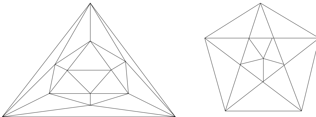
Figure 2.2: The graph I (the icosahedron) and the graph I^- .
