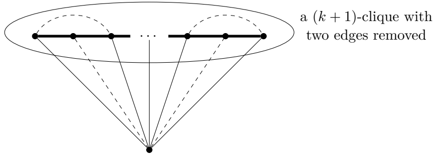
Figure 4.7: An extremal graph of \mathcal{J}_k with its connected edge-identifying code
