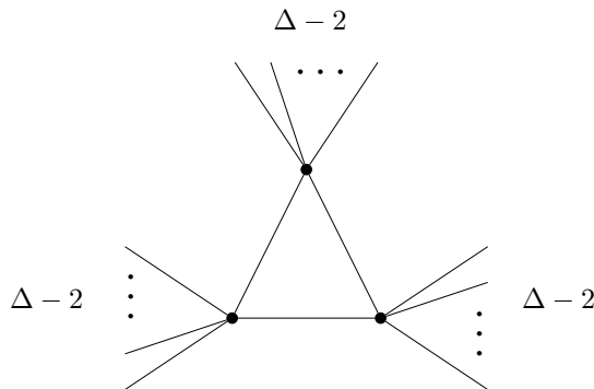
Figure 3.20: Example of outerplanar graph such that \chi'_s(G) = 3\Delta - 3 .
