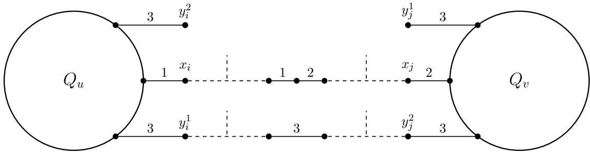
(b) Connecting two vertex gadgets in G'
