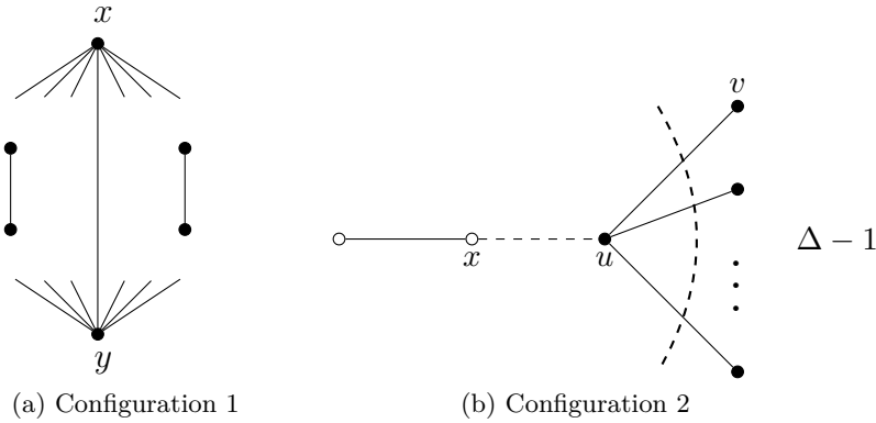
Figure 3.19: Forbidden configurations
