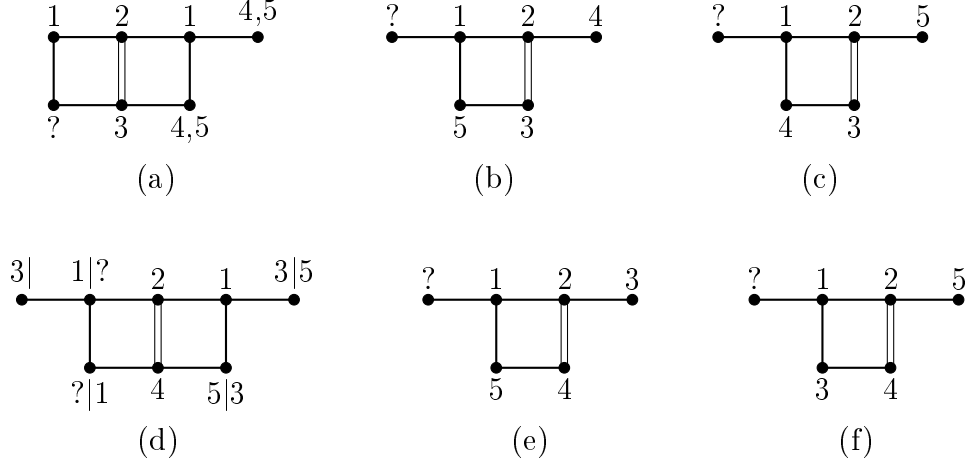
Figure 20: Configurations for the proof of Lemma 4 (cont.).
