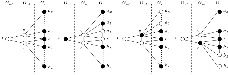
Figure 2: Configurations of Rule R1.
