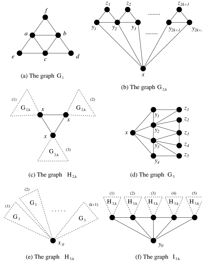
Figure 1: Impossibility results for outerplanar graphs.
