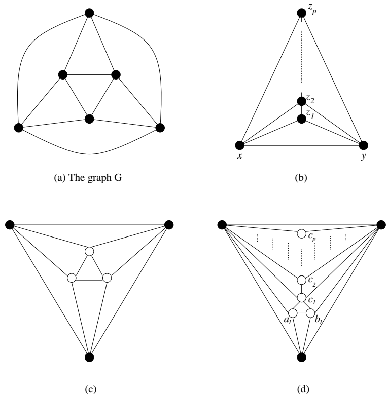
Figure 3: Impossibility results for planar graphs.
