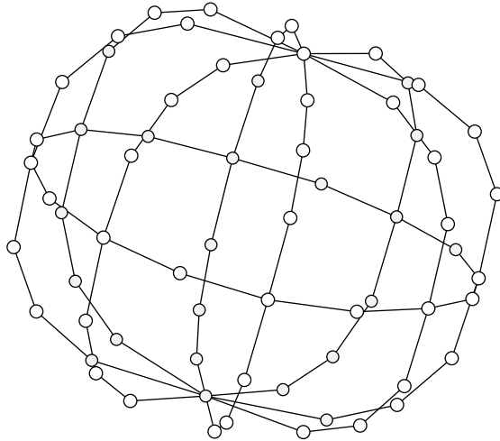
Figure 5: The planar graph embedded on a sphere for D = 8 such that \gamma_4(G) = 4 .
