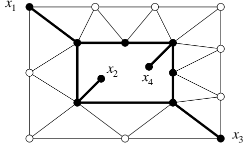
Figure 1: A plane graph G with a 4-gon H for k = 2 (bold edges).
