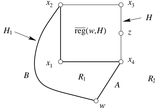
Figure 3: A node w' \notin \Gamma_k(H') has to belong to R_1 or R_2 .
