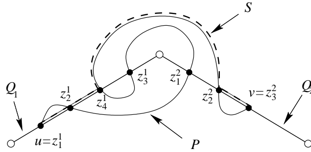
Figure 2: The simplified path S of P on Q_1 \cup Q_2 .
