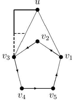
(a) d(v_1) = 3, d(v_3) = 3 or 4
