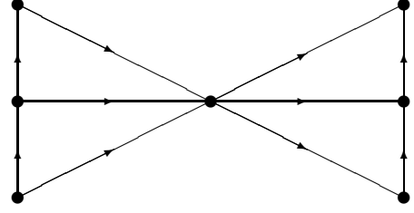
(b) An oriented graph with excess 4 and oriented chromatic number 7
