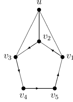
(b) d(v_1) = d(v_2) = d(v_3) = 3
