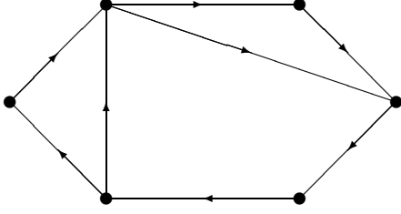
(a) An oriented graph with excess 3 and oriented chromatic number 6
