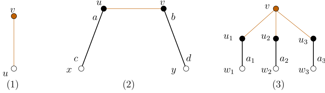
Fig. 3: Forbidden configurations for the proof of Theorem 11
