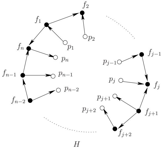
Figure 3: Configuration for the subcase 2.(d).iii.B
