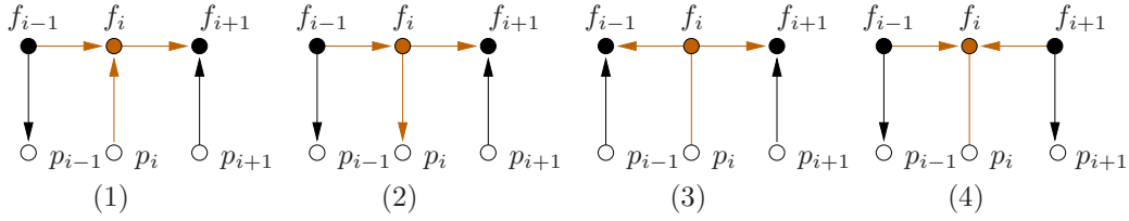
Figure 2: Configurations for the case 2.(b)
