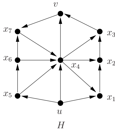
Figure 4: A Halin graph with oriented chromatic number 8
