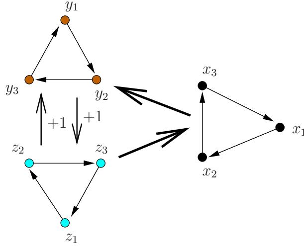
Figure 1: The graph G_9
