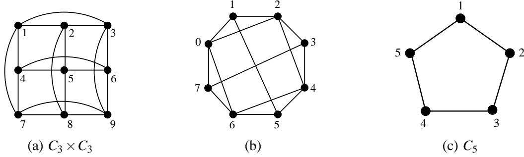
Fig. 1. Construction of the three target graphs T_9 , T_8 , and T_5 .
