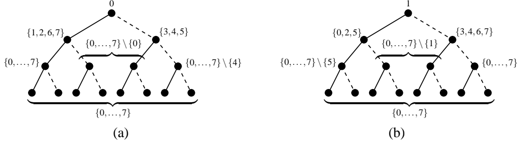
Fig. 2. The vertices of T_8 reachable from 0 and 1 by each (0, 2) -mixed k -path with 1 \leq k \leq 3 .
