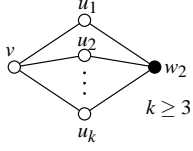
Fig. 5. A vertex v s.t. d(v) \geq 3 and D_4^H(v) = 1 .
