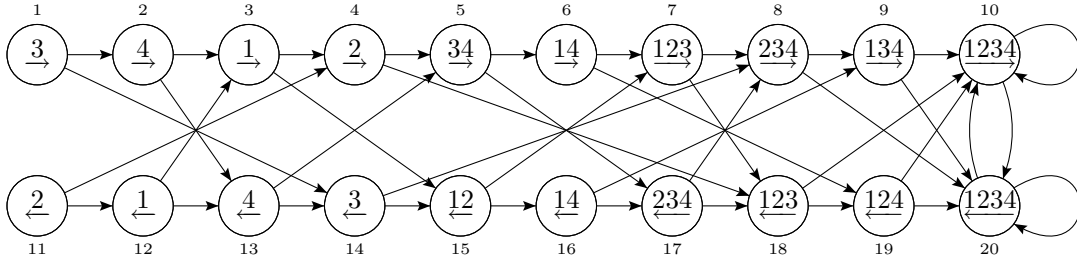
Figure 2: Automaton \mathcal{A} of Lemma 6
