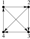
Figure 1: The tournament T_4
